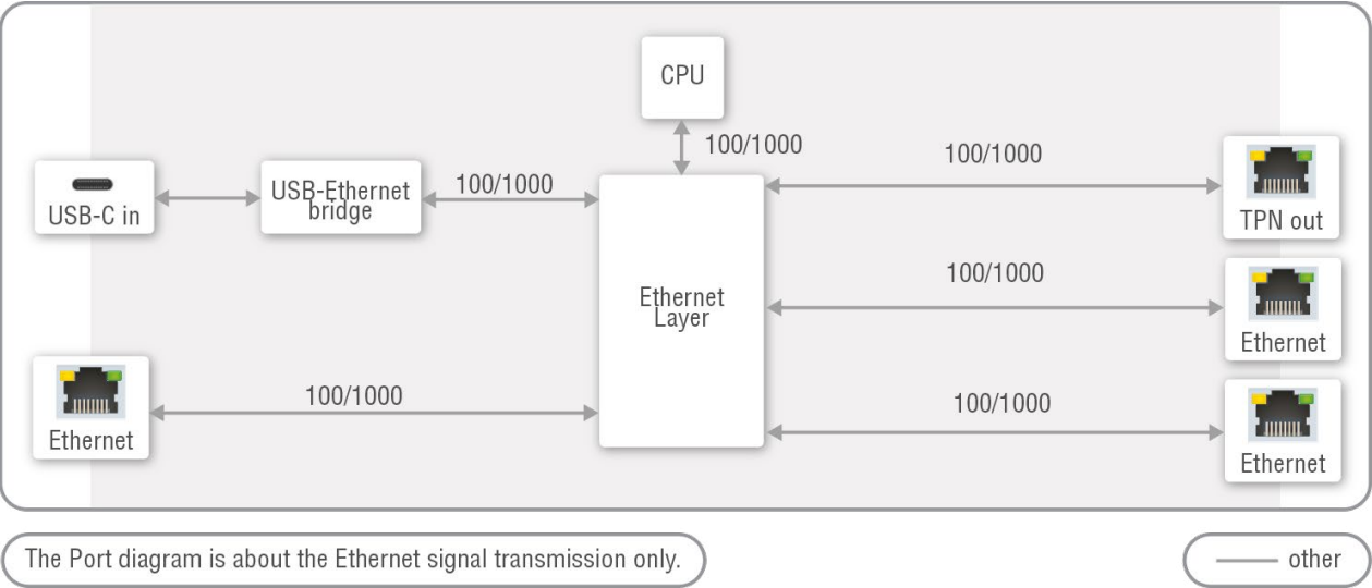
Ethernet Port Diagram (DCX-3x1-TPN-TX10)
