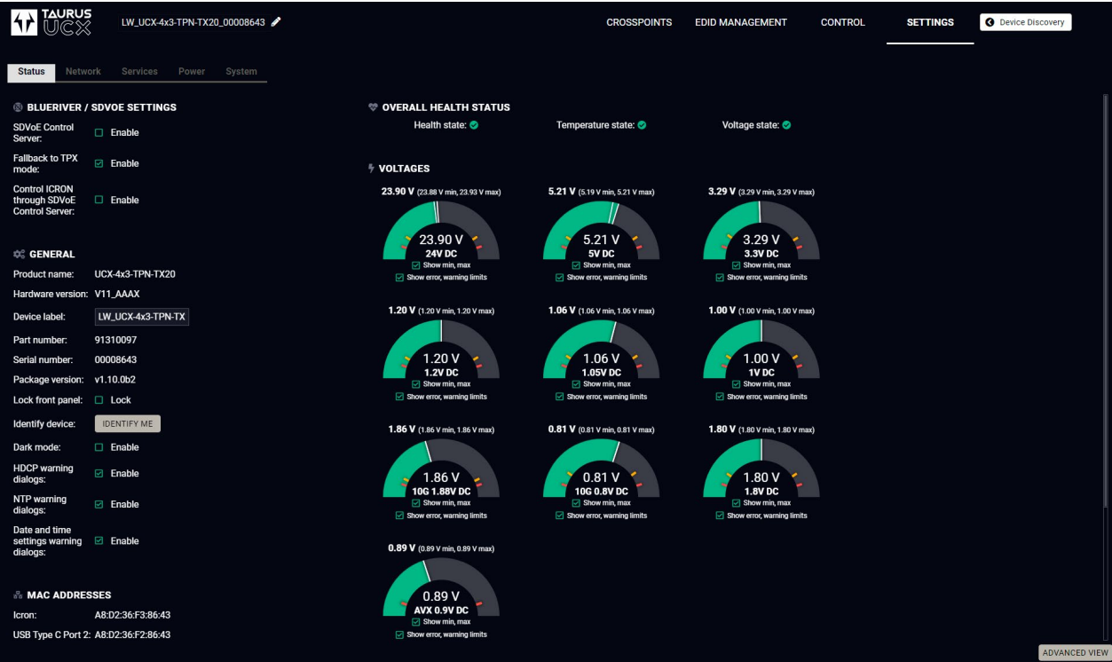
TX Status tab in the Settings menu
