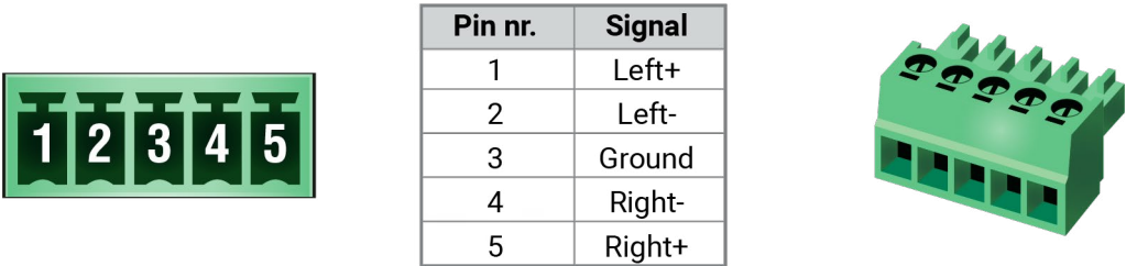
Analog audio connector and plug pin assignments
