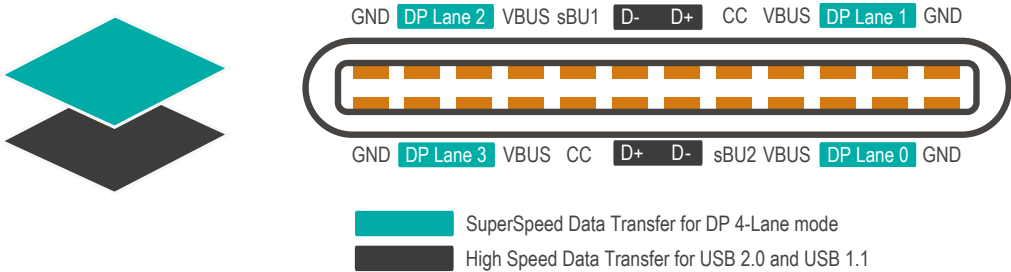
The pinout of the USB-C connector
