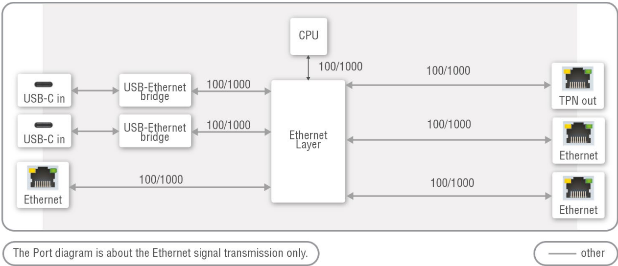
Ethernet Port Diagram (UCX-4x3-TPN-TX20)
