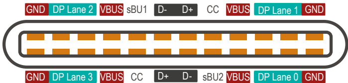
USB-C pinout in DP Alt mode
