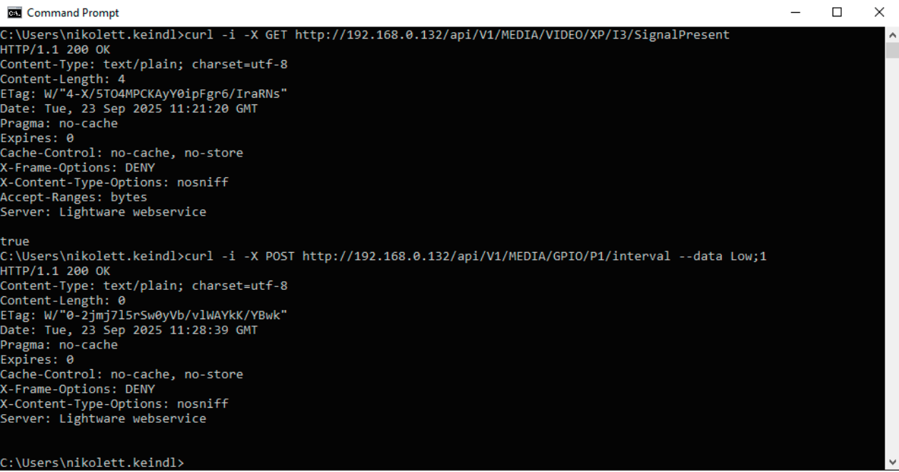
REST API communication in a command line window
