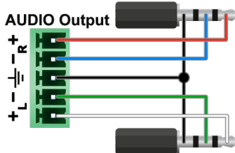
Phoenix - 2 x 6.3 (1/4") TRS
