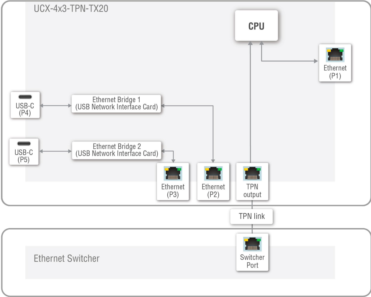
Dedicated VLAN preset with UCX-4x3-TPN-TX20 connected to an Ethernet switch
