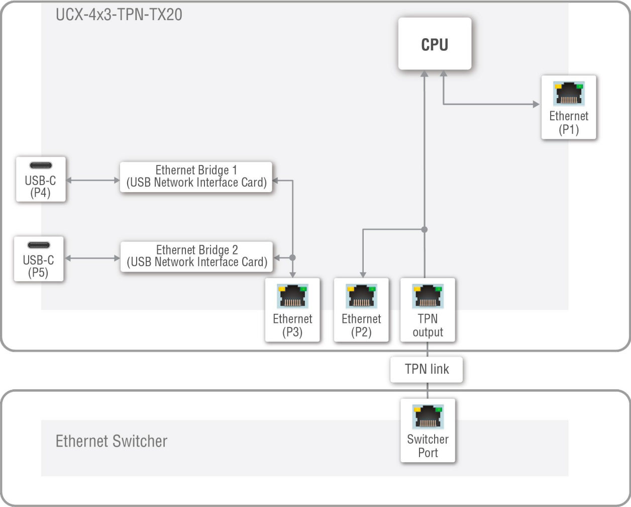
Separated BYOD VLAN preset with UCX-4x3-TPN-TX20 connected to an Ethernet switch
