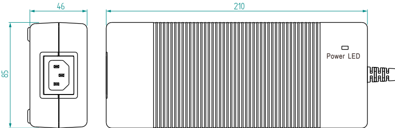
PSU-24VP3-220 (220W PSU for UCX-4x3-TPN-TX20)
