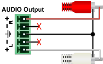
Phoenix - 2 x RCA
