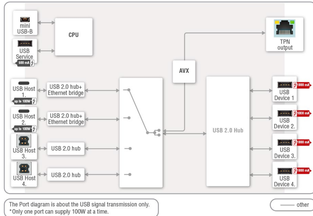
USB Port Diagram (UCX-4x3-TPN-TX20)
