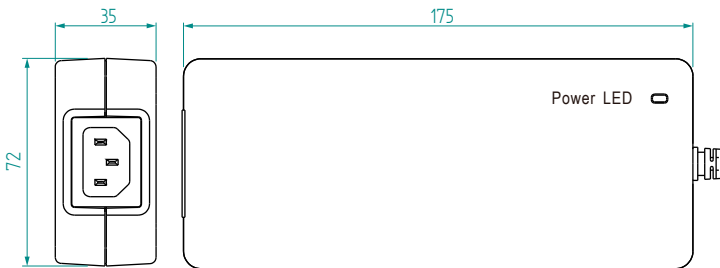
PSU-24VP3-160 (160W PSU for UCX-2x1-TPN-TX20)
