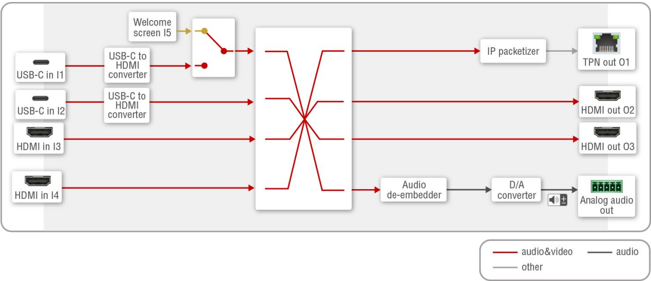
Video and Audio Port Diagram (UCX-4x3-TPN-TX20)
