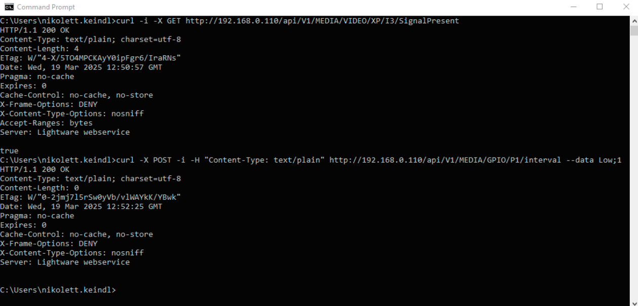
REST API communication in a command line window
