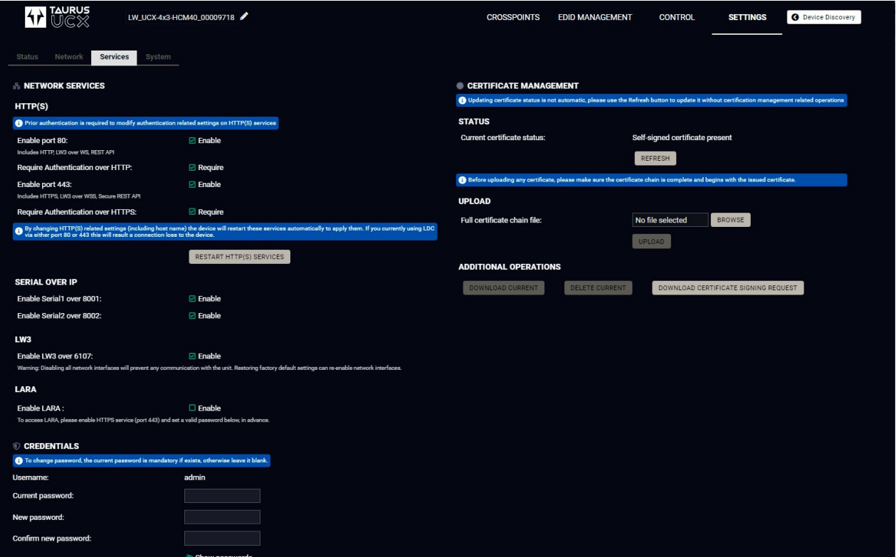
Services tab in the Settings menu
