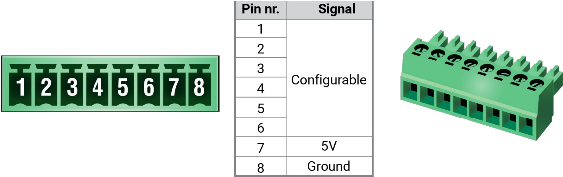
GPIO connector and plug pin assignments
