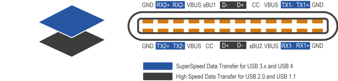
The pinout of the USB-C connector
