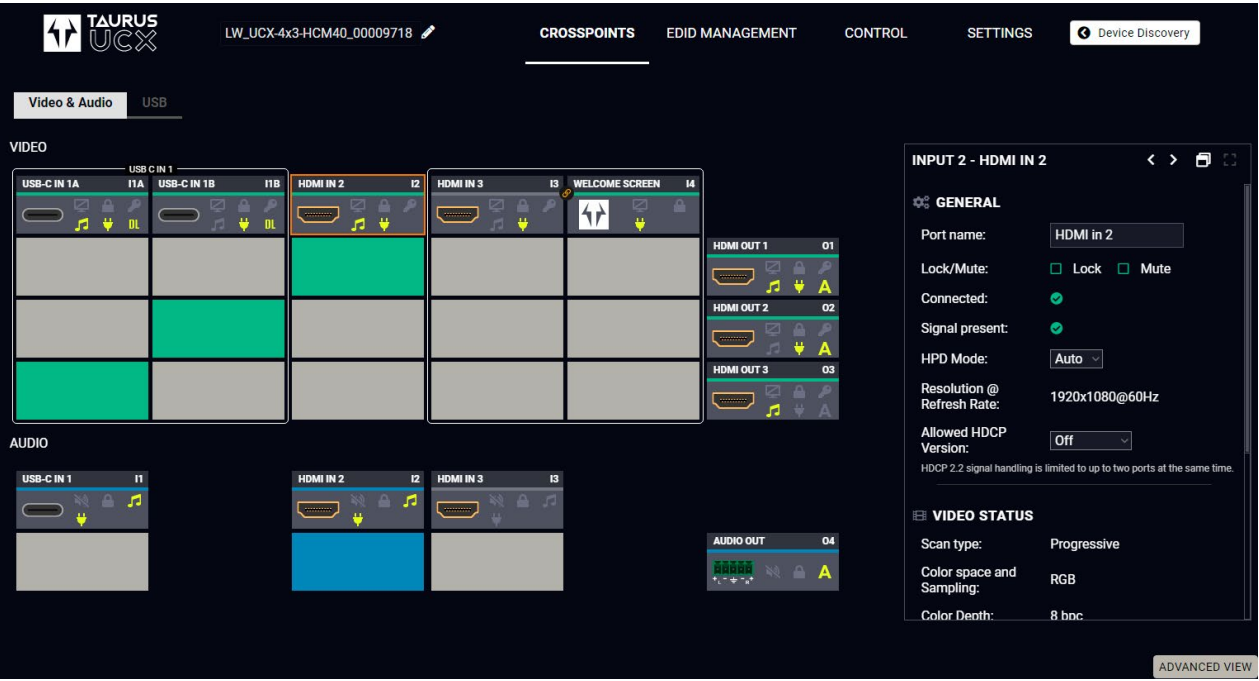
The Main window – Displayed in LDC
