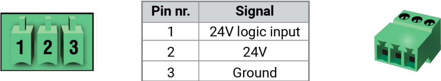
OCS connector pin assignments
