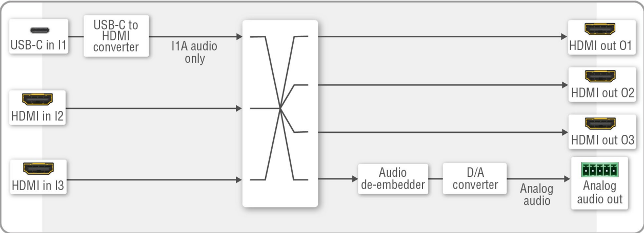
Audio Port Diagram
