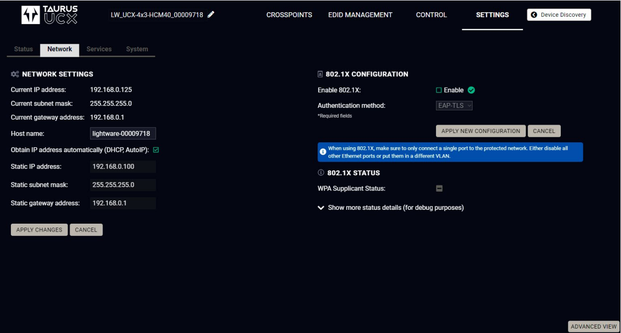
Network tab in Settings menu
