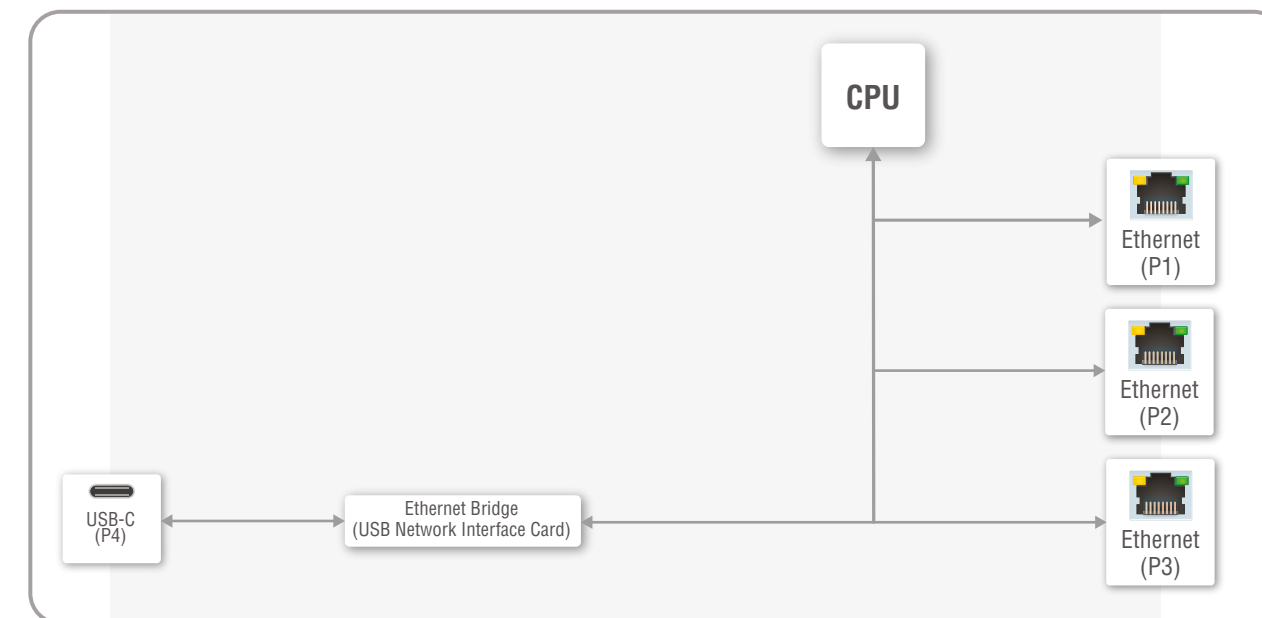
Transparent VLAN preset in UCX-4x3-HCM40
