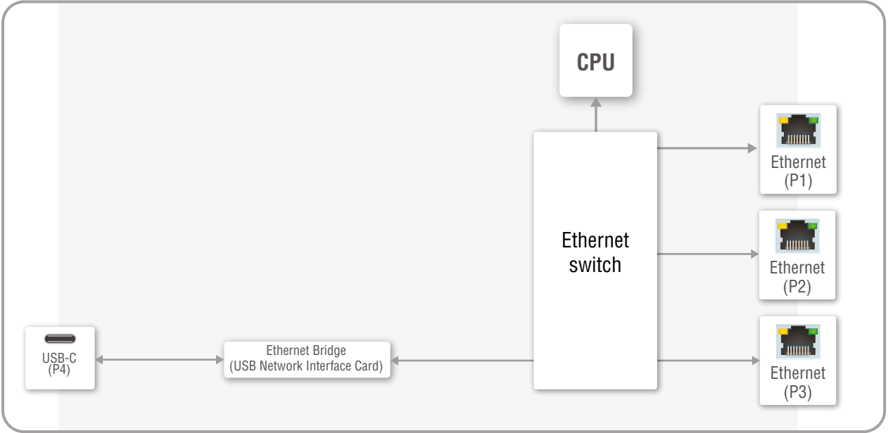
Custom VLAN preset in UCX-4x3-HCM40
