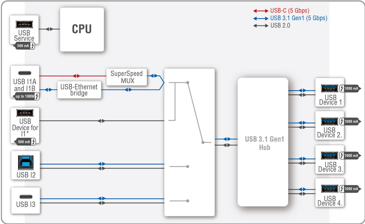
USB Port Diagram
